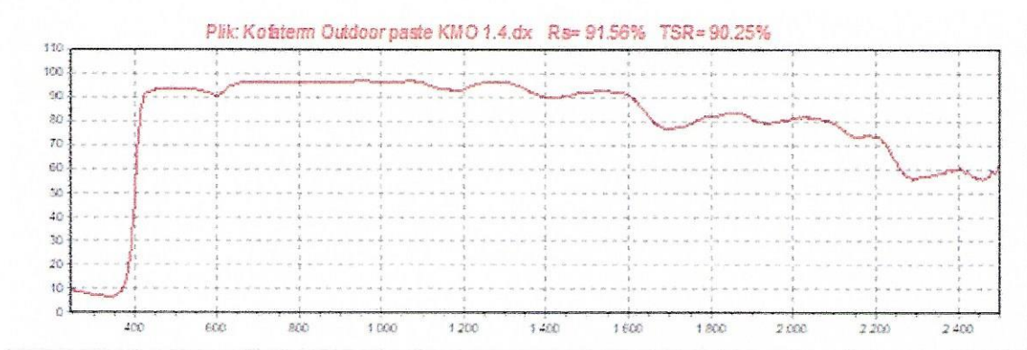
Fig. 1. The spectrum in the solar radiation range of the coating Kofaterm Outdoor Paste
