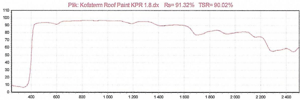
Fig. 1. The spectrum in the solar radiation range of the coating Kofatern Roof Paint
